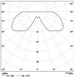
1xG.12-70W HIT
