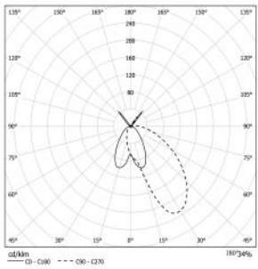
1xG.12-150W HIT
